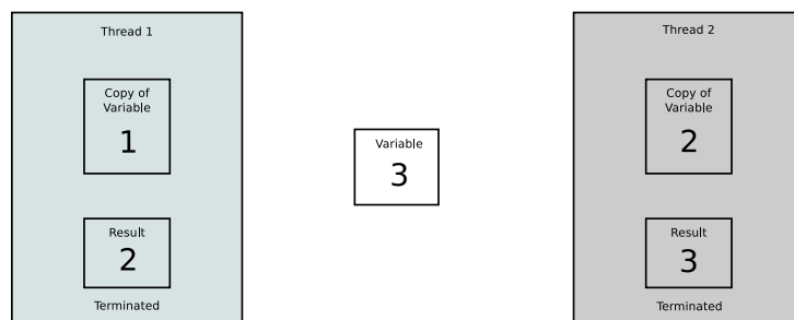
Figure 127: How mutex works (8/8)
